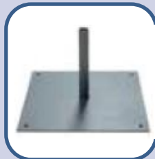
5mm Steel Plate 40x40cm
